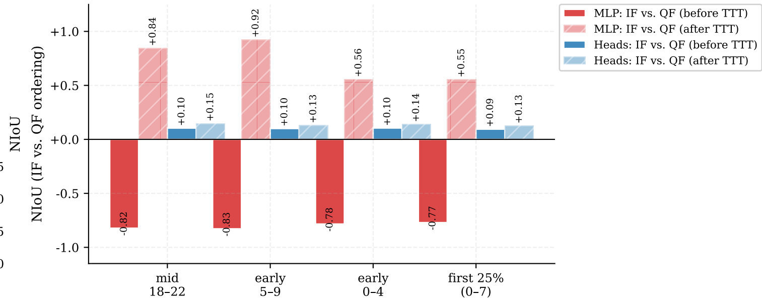
(b) MLP misalignment (IF vs. QF) resolved across all adaptation windows
