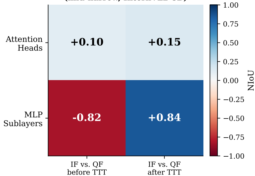
(a) IF vs. QF alignment (mid-narrow, InternVL2-8B)
